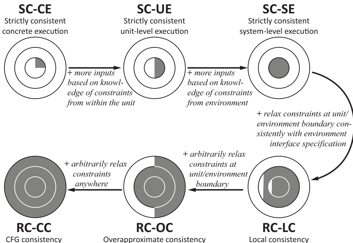
Figure 2.5 – Different execution consistency models cover different sets of feasible paths. The SC-CE model corresponds to concrete execution. The SC-UE and SC-SE models are obtained from the previous ones by using increasingly more information about the system, to explore increasingly bigger sets of concrete paths. The RC-LC, RC-OC and RC-CC models are obtained through progressive relaxation of constraints.
